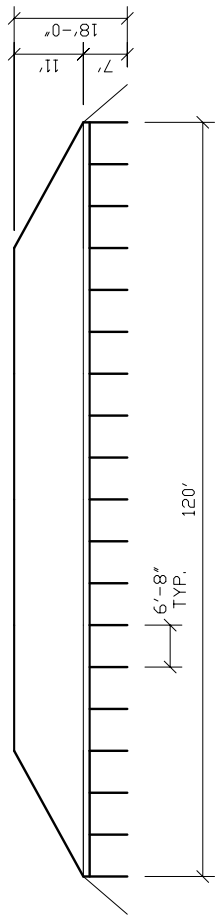
SIDE ELEVATION
